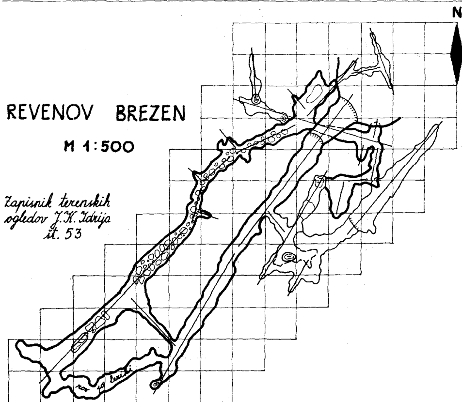
Sl. 2. Revenov brezen, poglavitni rovi potekajo ob prelomih ali razpokah Fig. 2. Cave Revenov brezen, the principale channels pass along faults or joints
